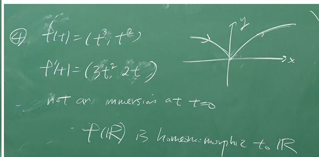
Figure 2: Examples from Example 2.4
